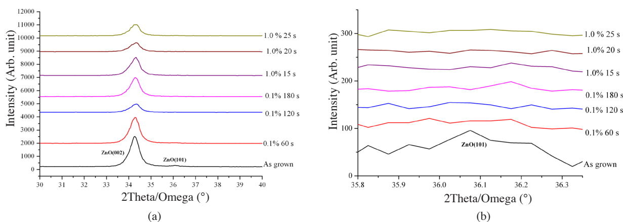
FIGURE 1. XRD patterns of as-grown ZnO and ZnO thin films etched in 0.1% and 1.0% HNO 3 solutions
